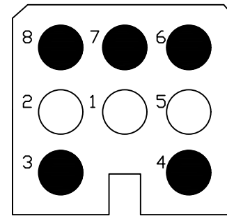
FACE VIEW
